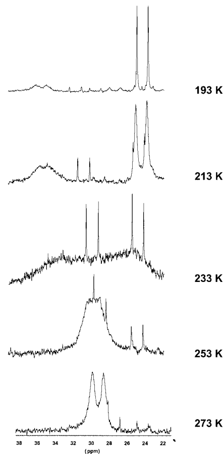
Figure 1. Low-temperature ^{31}\text{P}\{^1\text{H}\} NMR spectra of [\text{Rh}(\text{CO})(\text{I})_2][\text{BF}_4]
