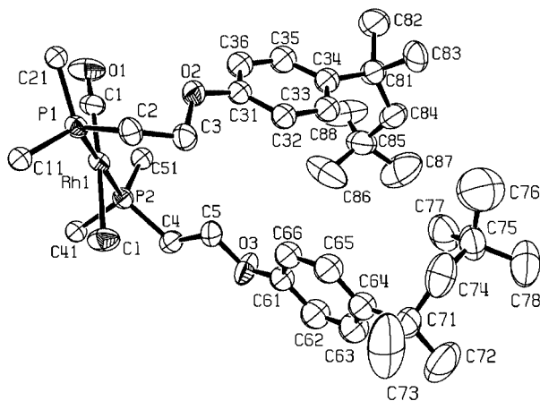
Figure 2. ORTEP diagram of \text{trans-}[\text{Rh}(\text{CO})(\text{1})_2\text{Cl}] showing the atom numbering scheme. The phenyl rings bonded to phosphorus have been omitted
