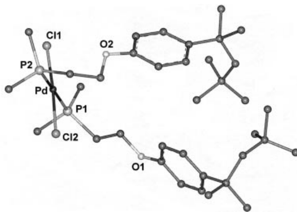
Figure 3. View of the molecular structure of \text{trans-}[\text{PdCl}_2(\text{1})_2] . The phenyl rings bonded to phosphorus have been omitted
